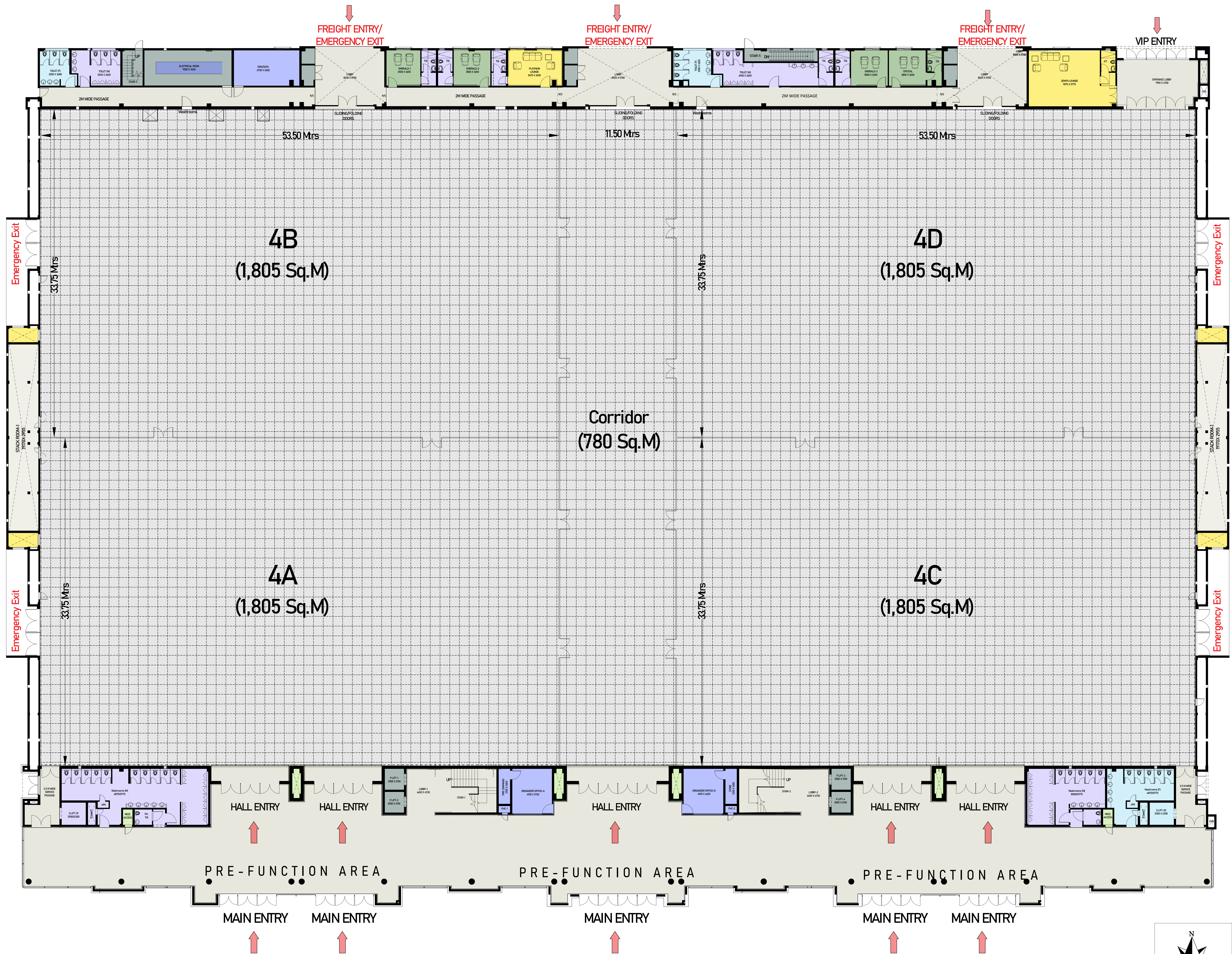
HALL 04 LAYOUT
